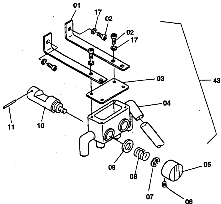
Control Valve (OP-S)
